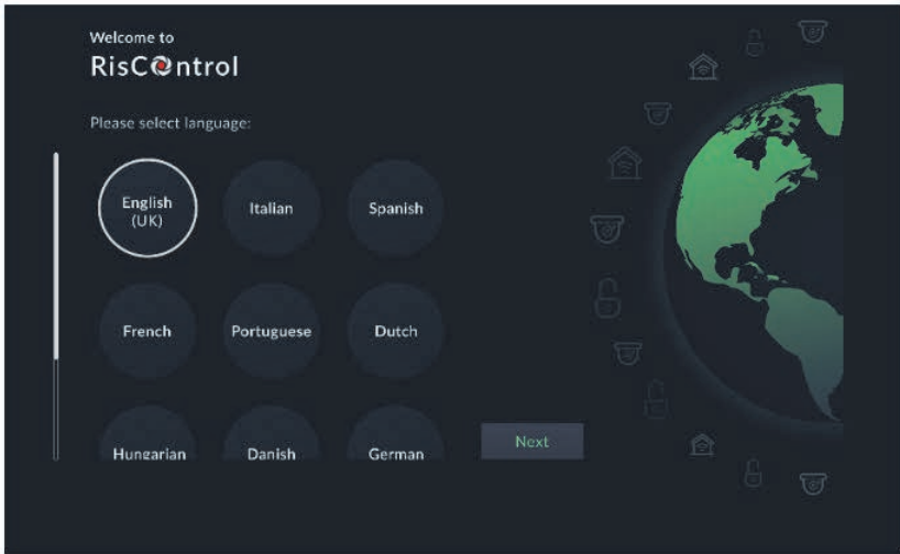
Figure 2: Welcome Screen
