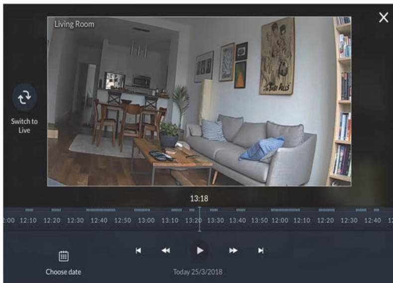
Figure 46: Playback Screen
