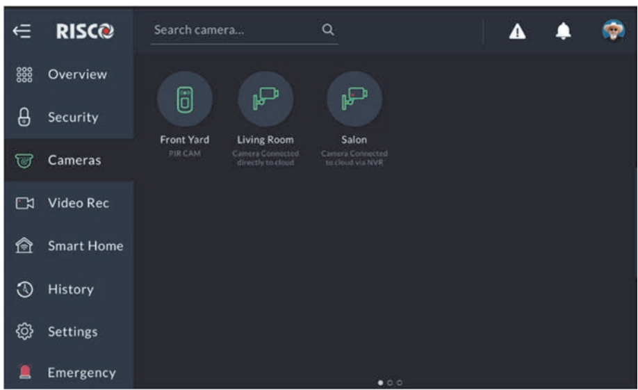
Figure 35: Cameras Screen
