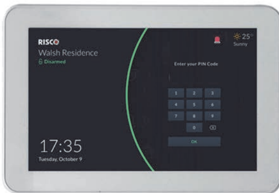
Figure 19: Lock Screens
