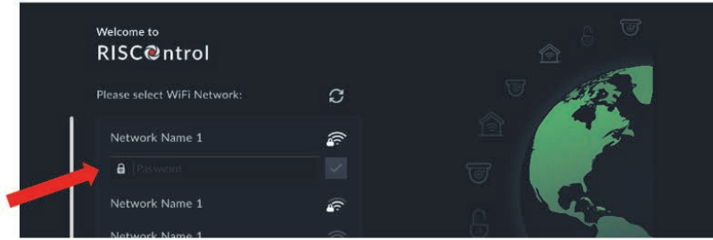
Figure 5: Enter Password
